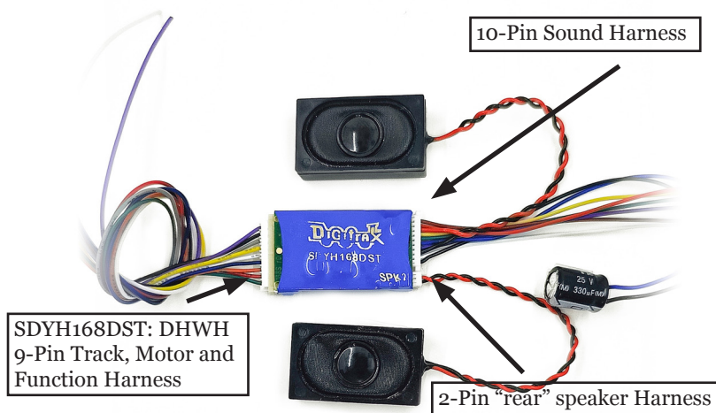
Figure 1: SDYH168DST Decoder Components
