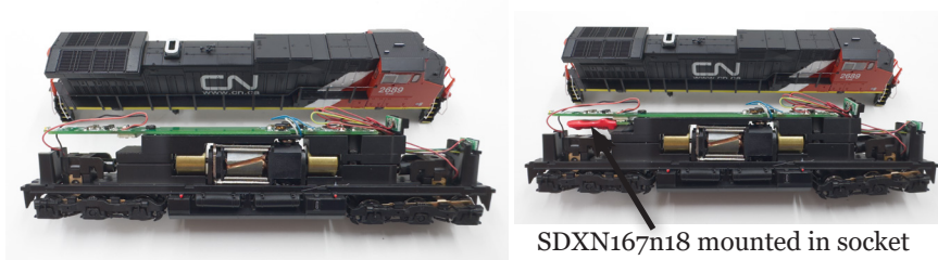
Figure 3: ScaleTrains C44-9 SDXN167n18 decoder installation
