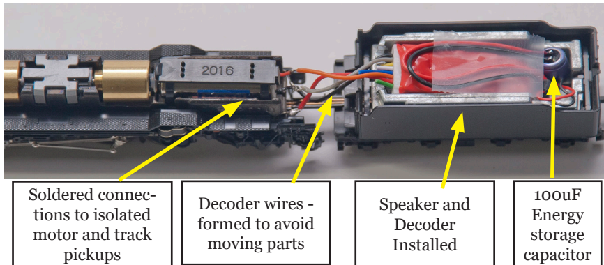
Figure 2: SDXN147PS: Wired Install example in Steam Locomotive
