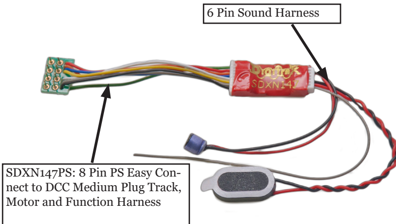
Figure 1: SDXN147PS Decoder Connections
