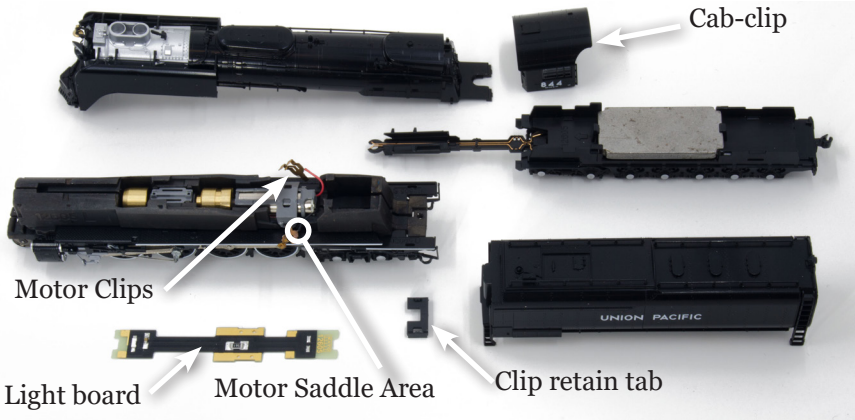
Figure 1: SDXN147K4: Locomotive with light board and motor clips removed
