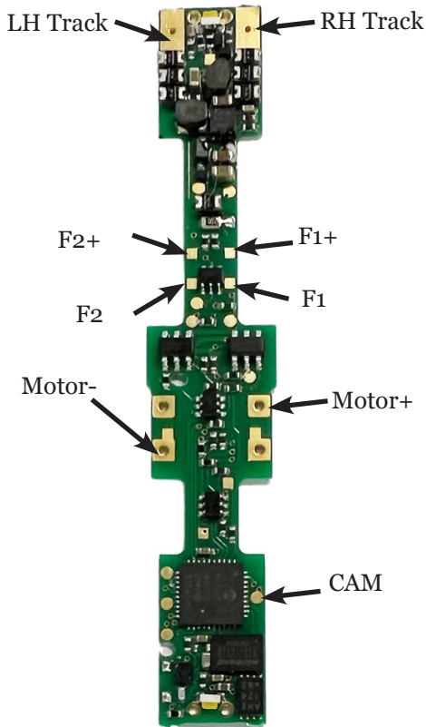
Figure 3: SDXN147K4: connection diagram
