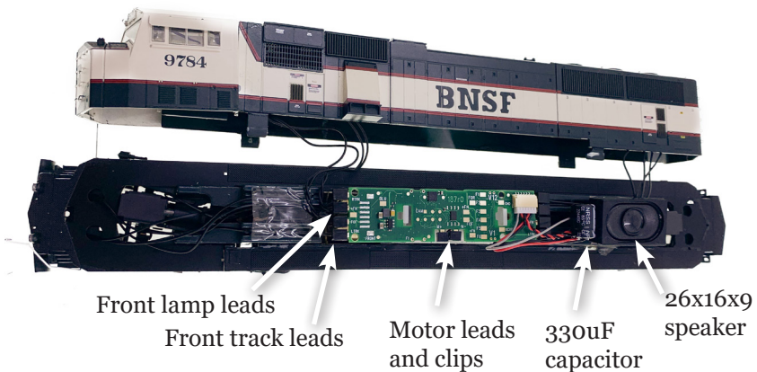
Figure 1: SDXH187Ao: Locomotive with decoder installed.
