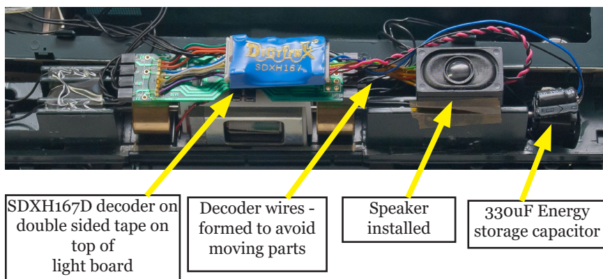
Figure 2: SDXH167D: Install in an Athearn 9-Pin plug locomotive.
