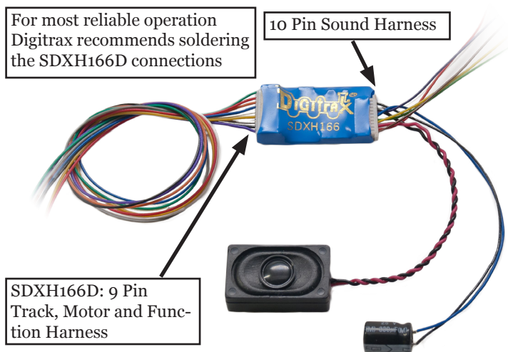
Figure 1: SDXH166D Decoder Connections
