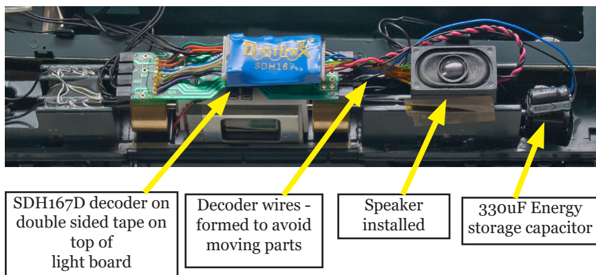
Figure 2: SDH167D: Install in an Athearn 9-Pin plug locomotive.
