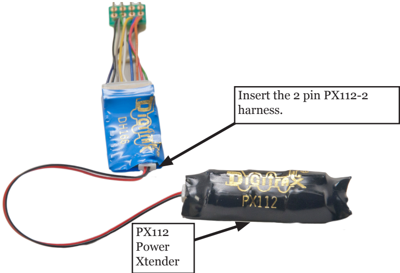
Figure 2: Installing the PX112-2 Power Xtender
