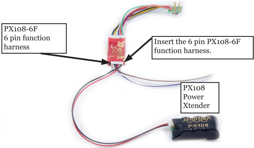
Figure 2: Installing the PX108-6F Power Xtender
