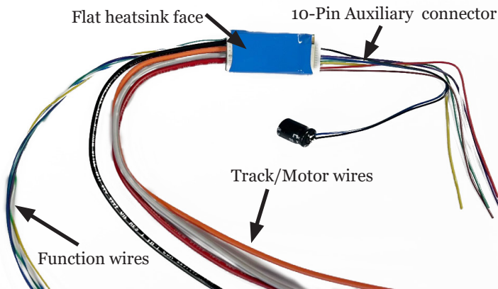
Figure 1: DO487 Decoder showing Track/Motor, Function wires, Auxiliary connector, heatsink face and 330uF capacitor.
