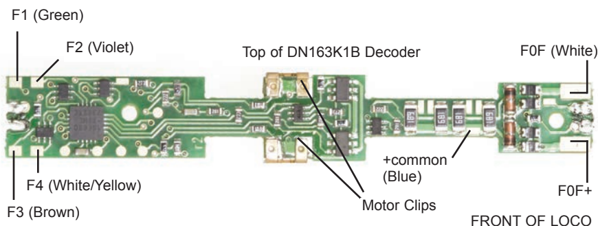
Figure 5: Connecting More Functions to Your DN163K1B Decoder
