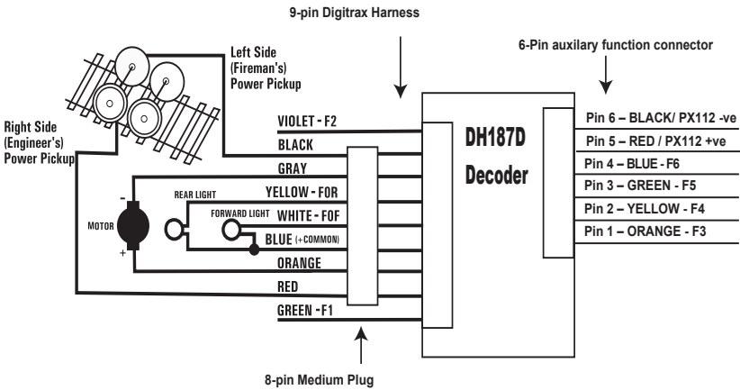
Figure 2: DH187PS: connection diagram
