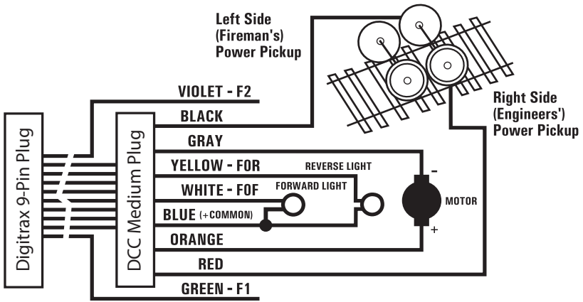
Figure 2: DH127P: connection diagram
