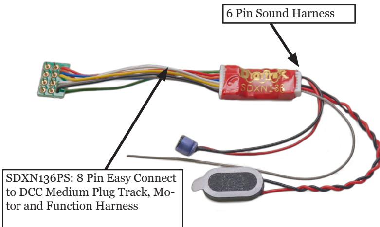
SDXN136PS showing 8 Pin Sound Harness with 8 Ohm 10 mm x 18 mm Oval speaker and 100uF capacitor
