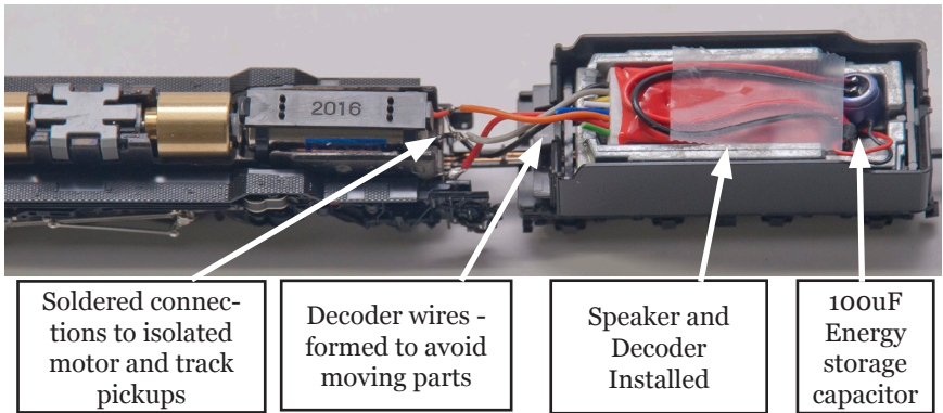
Figure 2: SDXN136PS: Wired Install example in Steam Locomotive
