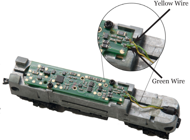
Figure 4: Solder headlight wires, secure new decoder with original screws
