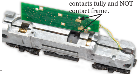
Figure 3: Unscrew, unsolder and remove standard lightboard.
