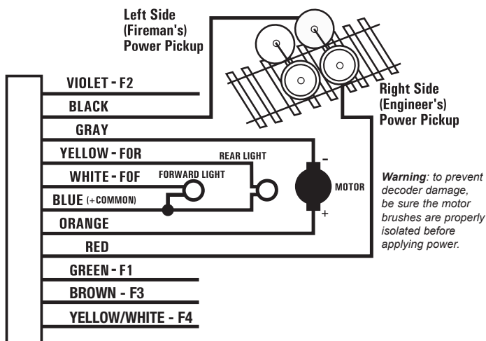
Figure 1. DN163 Wiring Diagram
