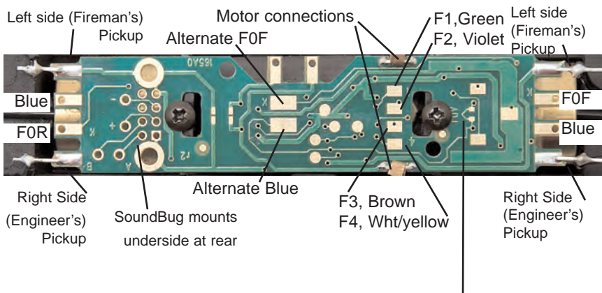
Figure 5. DH165K0 Decoder Function Outputs (front of loco to the right)
