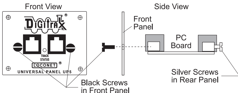
Figure 1. Panel Installation
