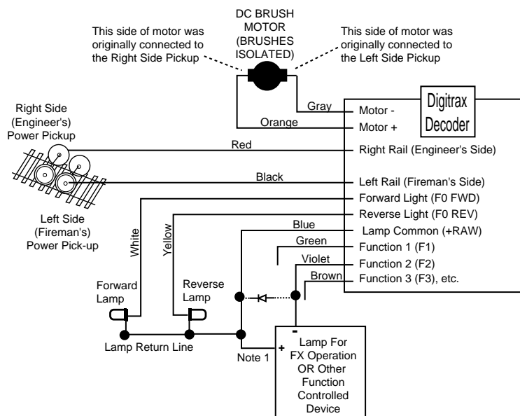
Figure 1: Digitrax Decoder Wiring Diagram
