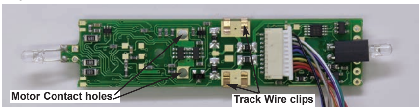
Figure 1: SDH164K1A Decoder
