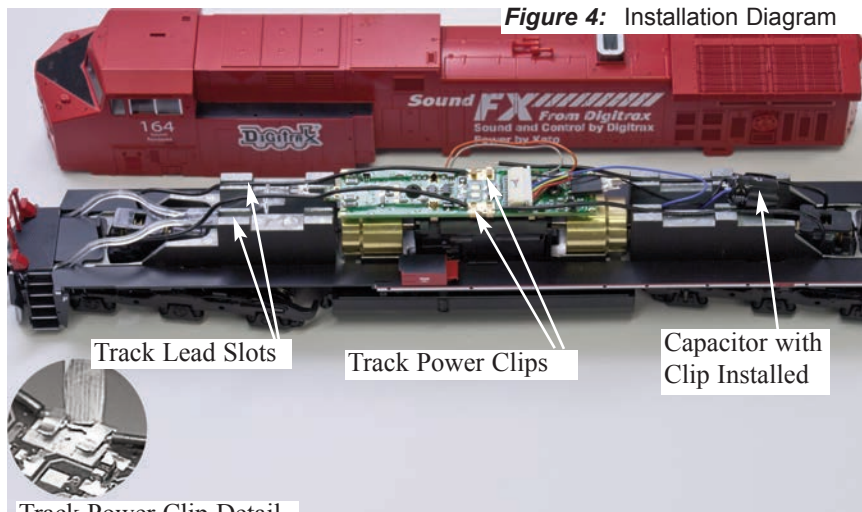
Track Power Clip Detail
