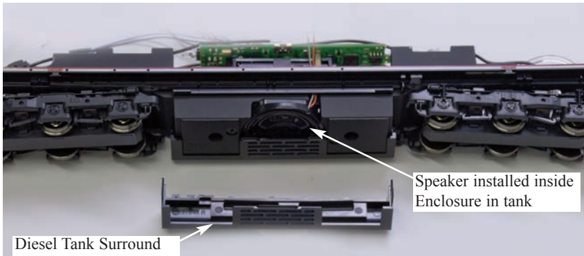
Figure 3: Speaker Installation Diagram
