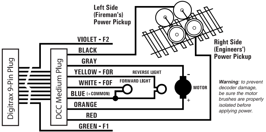
Figure 1. DHWHP5 Wiring Diagram showing pin outs for DCC plug.
