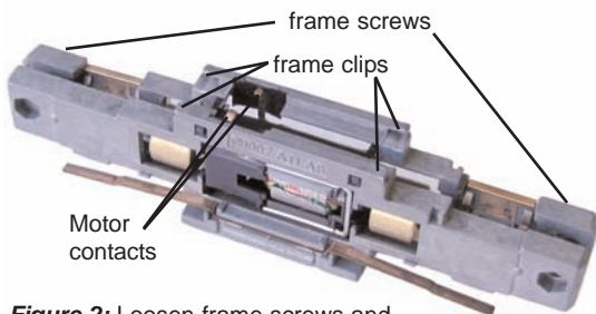
Figure 2: Loosen frame screws and remove light board
